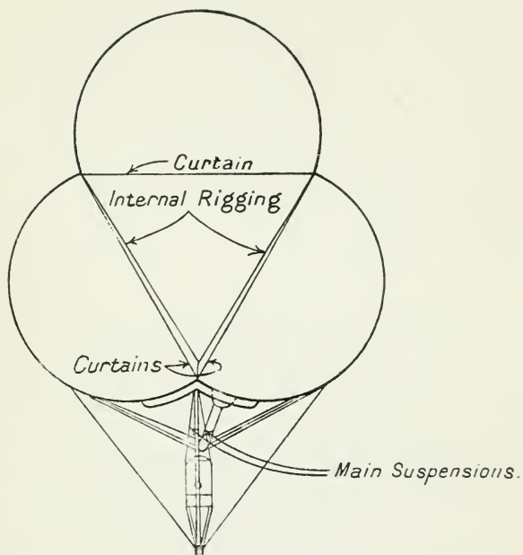
CROSS SECTION OF COASTAL AIRSHIP
